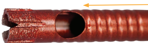
Relief slot for core removal
